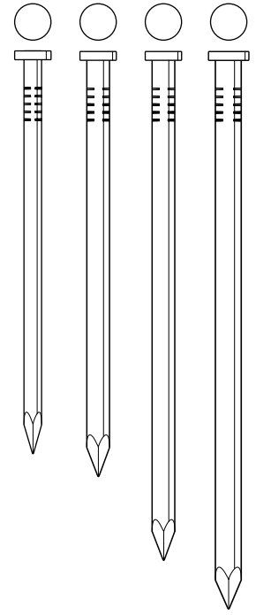
.113", .120", .131", .148" 2 3/8" - 3 1/2"
