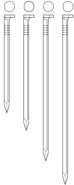
.113", .120", .131", 135" 2" - 4"
